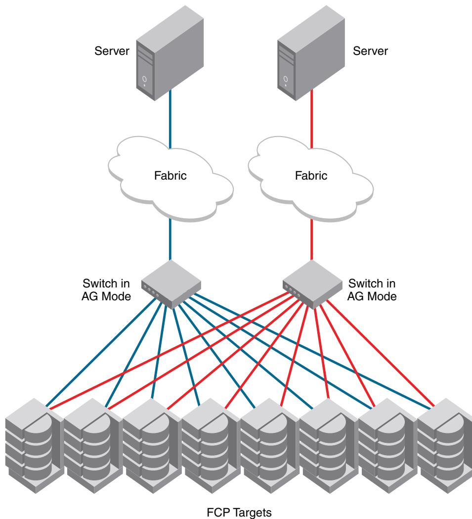
FIGURE 15 Target aggregation
